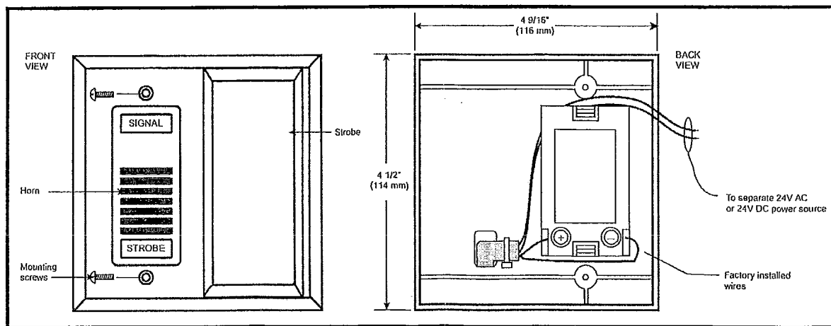
Figure 1. Details of Horn/Strobe
